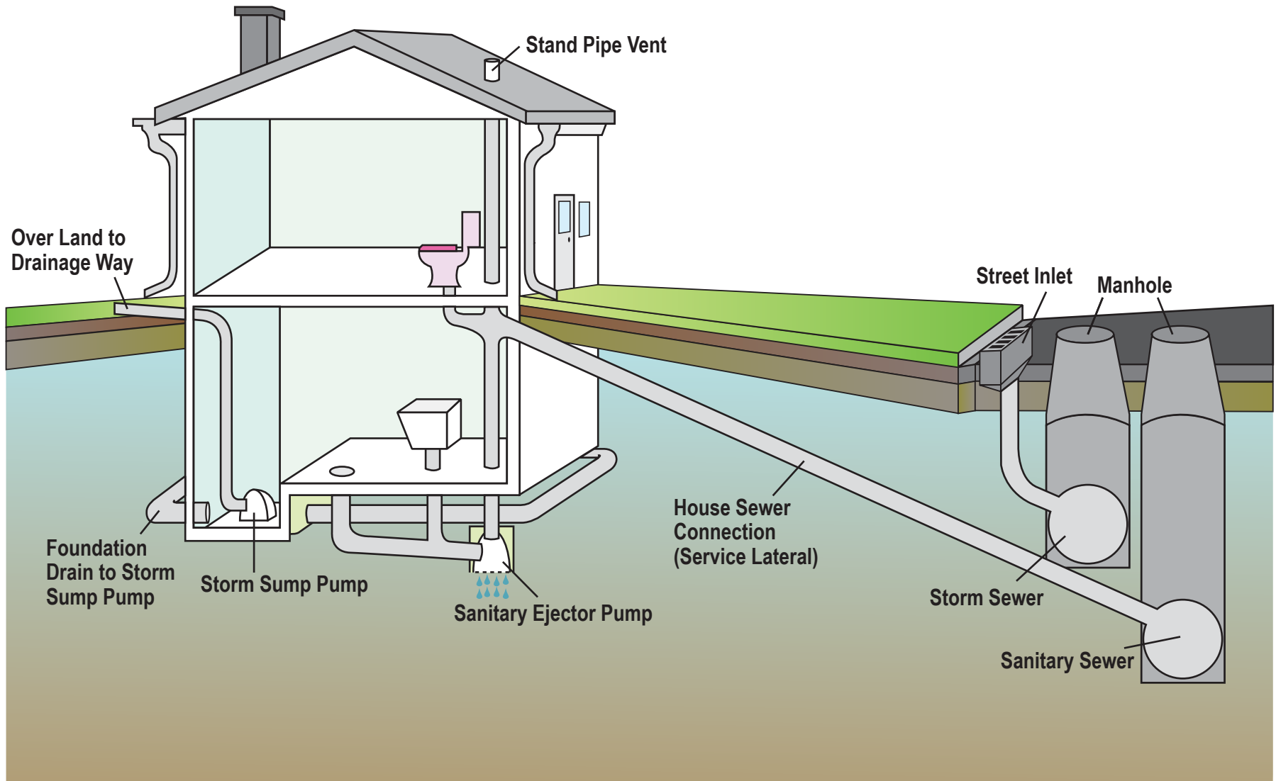
Combination sump to separate sanitary
